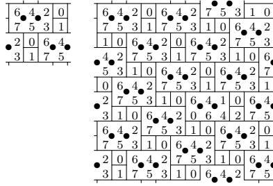
Figure 4: First two even-weight cases: M(0) and M(011)
