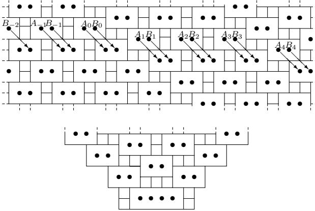
Figure 1: Illustrations for Theorem 1
