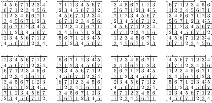
Figure 11: Case r = 3
