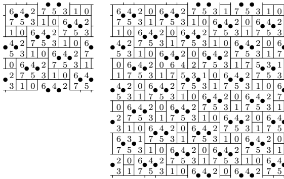
Figure 5: First two odd-weight cases: M(1) and M(01)
