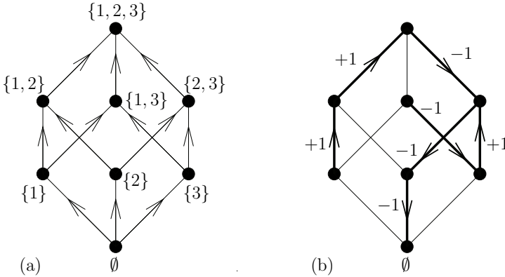
Figure 2: Calculating the signs \mu(e) of the edges of a spanning tree. (a) The oriented edges of Q_3 . Each edge is oriented in the direction of increasing cardinality. (b) The oriented edges of a spanning tree T and the resulting signs; the vertex labels have been omitted for clarity. Each edge of T is oriented towards the root at \emptyset , and the sign is +1 where this orientation agrees with the orientation in (a), and -1 where it disagrees. The tree has weight q_1^2 q_2^3 q_3^2 x_1^{-1} x_2^2 x_3 .
