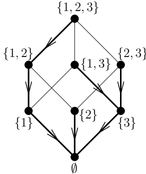
Figure 6: An upright spanning tree of Q_3 . The associated section \phi (see Section 4.3) is determined by \phi(\{1, 2, 3\}) = 3 , \phi(\{1, 2\}) = 2 , \phi(\{1, 3\}) = 1 and \phi(\{2, 3\}) = 2 .
