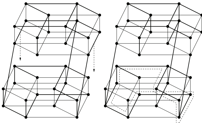
Figure 9: Parallel edge slides need not be independent, even when there are no more edge slides in that direction than expected. The figure on the left illustrates a spanning tree of the 5-cube, with some edges of the 5-cube omitted for clarity. The tree has three edges joining the upper and lower 4-cubes, and precisely two edges that may be slid from one 4-cube to the other. The figure on the right shows the result of sliding both. This contains a cycle, indicated by the dashed line which shadows it.
