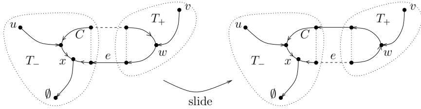
Figure 5: The effect of an edge-slide on orientations. Only those edges belonging to C \cap T_+ are reversed.
