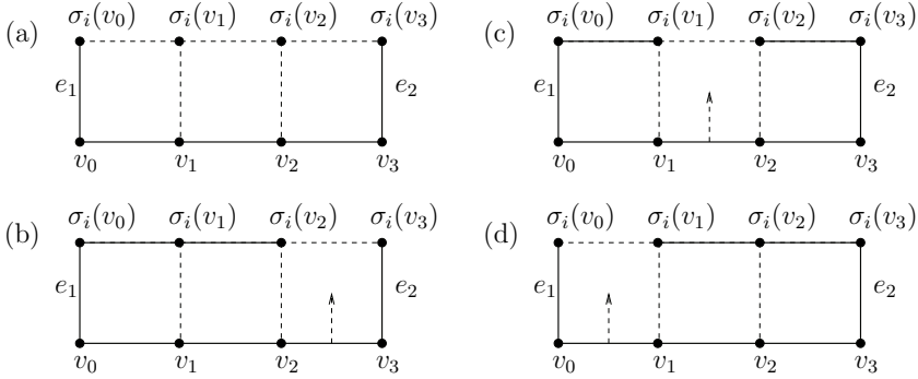
Figure 4: The case where P has length 3 in the proof of Lemma 2.
