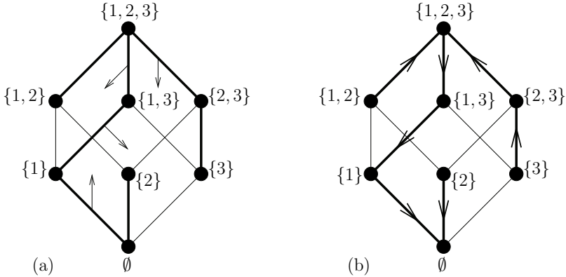
Figure 3: (a) The slidable edges in a certain spanning tree T of the three-cube. The edge (\emptyset, \{1\}) may be slid up in direction 2; the edge (\{1\}, \{1, 3\}) may be slid down in direction 1; the edge (\{1, 3\}, \{1, 2, 3\}) may be slid down in direction 3; and the edge (\{2, 3\}, \{1, 2, 3\}) may be slid down in direction 2. (b) The oriented edges of T (see Section 3.2). The edges (\{3\}, \{2, 3\}) , (\{2, 3\}, \{1, 2, 3\}) and (\{1, 2\}, \{1, 2, 3\}) are upward edges and the rest are downward.
