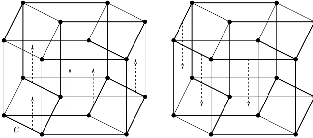
Figure 8: “Extra” edge slides when n = 4 . The tree on the left has only two vertical edges, but there are five edges (indicated with dashed arrows) on the path joining them that may be slid vertically. The tree on the right shows the result of sliding the edge labelled e at left. This now has three vertically slidable edges on the path joining the two vertical edges.
