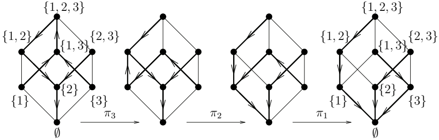
Figure 7: An example of the retraction \pi = \pi_1 \circ \pi_2 \circ \pi_3 . By successively carrying out all possible downward edges slides in directions 3, 2, 1 in turn we arrive at the upright tree on the right.
