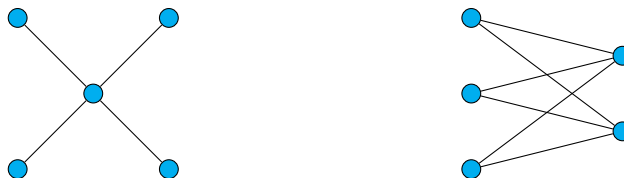
Figure 3.1: A star graph on 5 vertices and the complete bipartite graph K_{3,2} .
